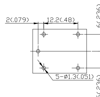
Drilling Plan (Bottom View)
