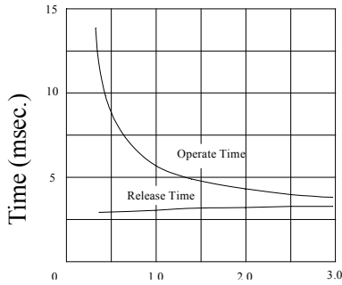
Timing
