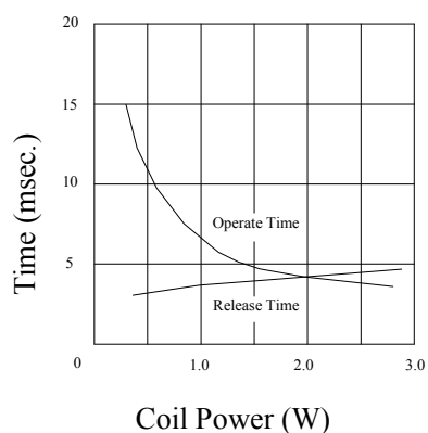
Timing
