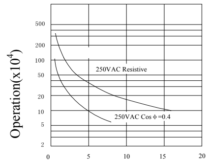
Life Curves
