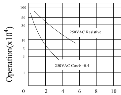
Life Curves
