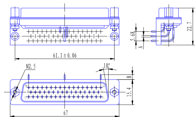
J18D-50P ( × ) outline size
