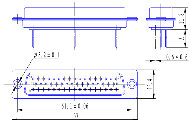
J18D-50PF179 ( × ) outline size
