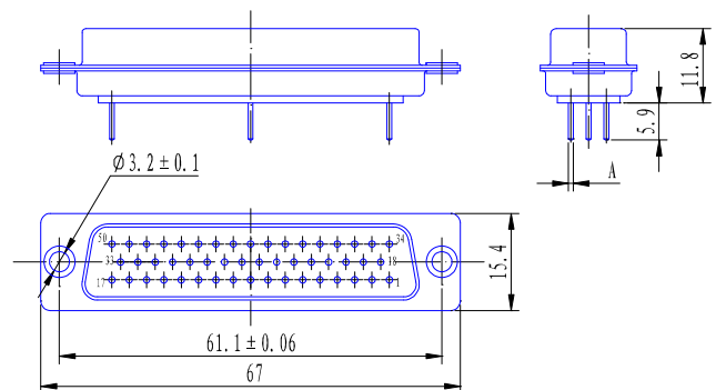
J18D-50P ( × ) outline size
